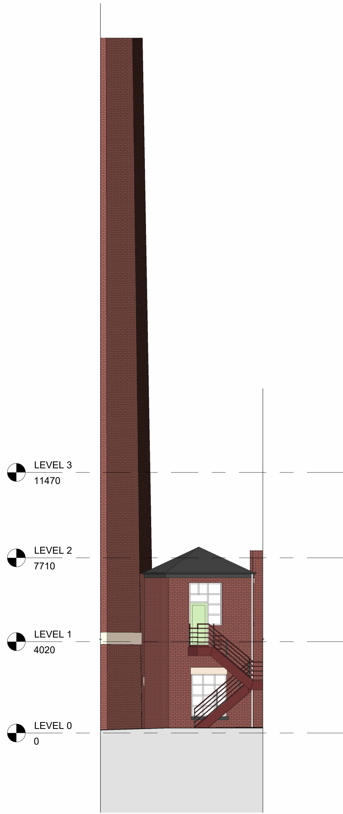
1 Albion Mill Rear - FRONT 1 - Proposed 1 : 100
