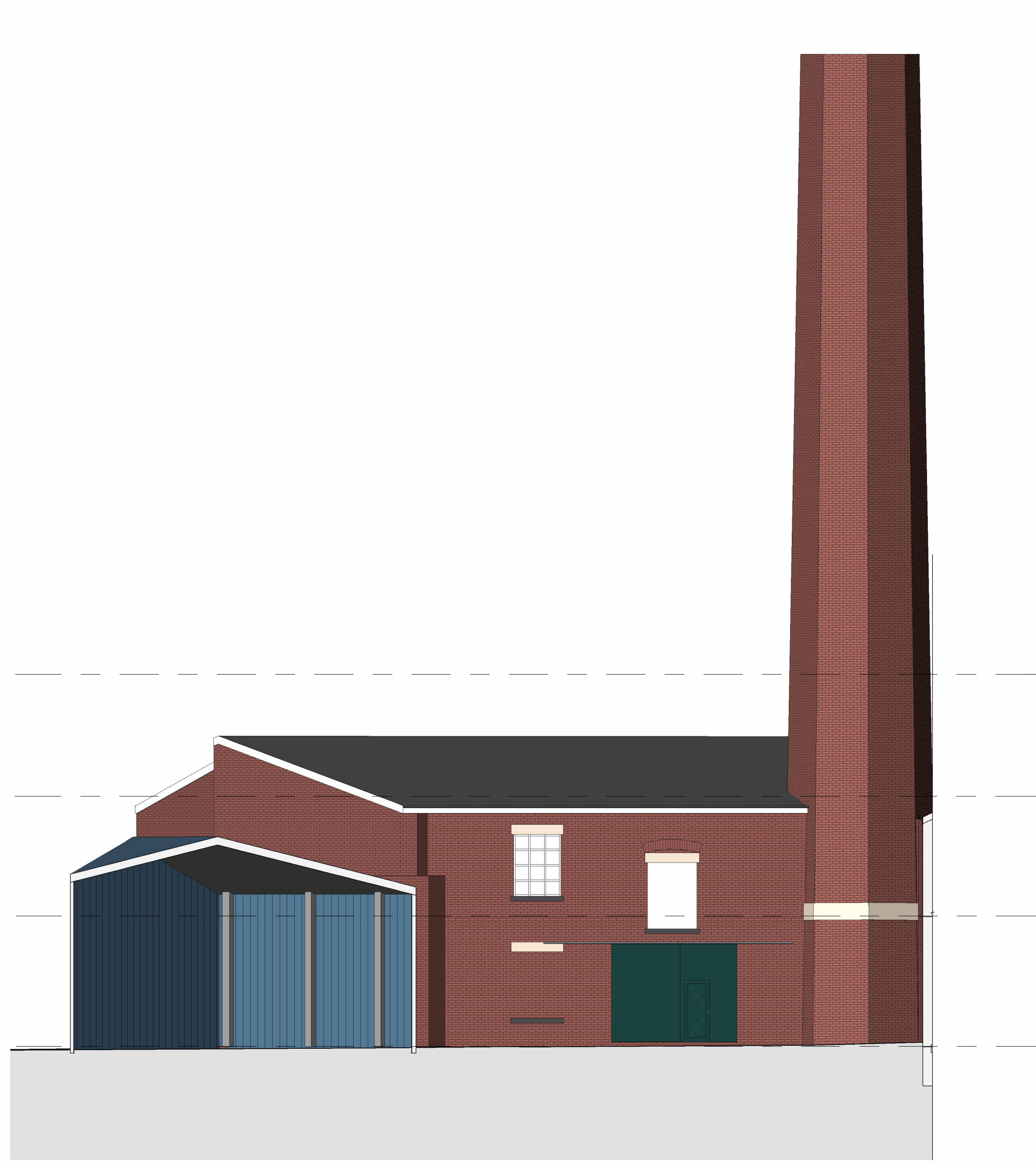
2 Albion Mill Rear - FRONT 2 - Proposed 1 : 100
