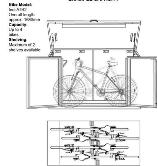
ACCESS BIKE SHED x4 EXAMPLE CAPACITY
