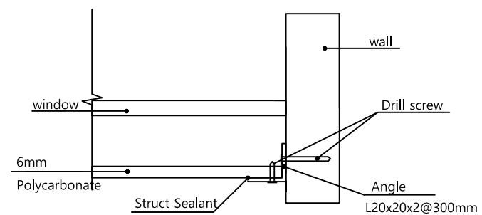
1-1 Panel Installation Detail
