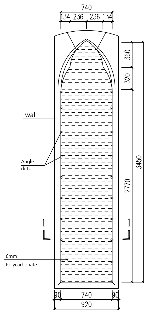
Polycarbonate elevation 1:25 (exterior)
