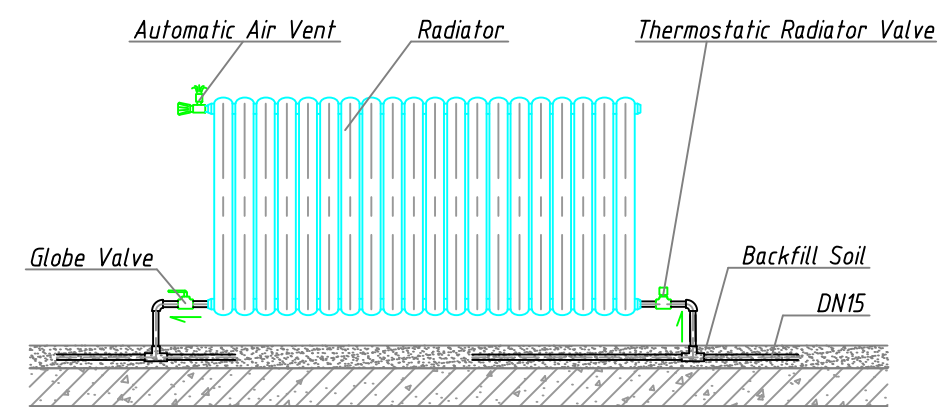
Radiator Detail Drawing
