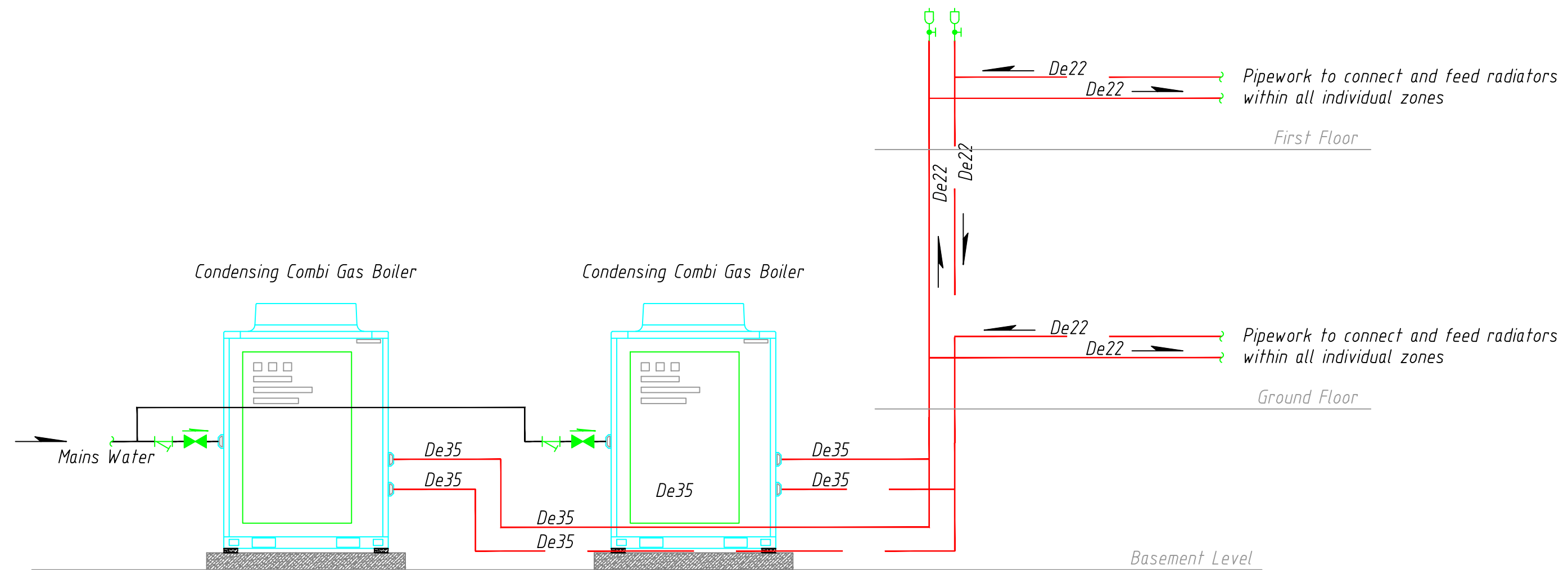
Heating System Schematic
