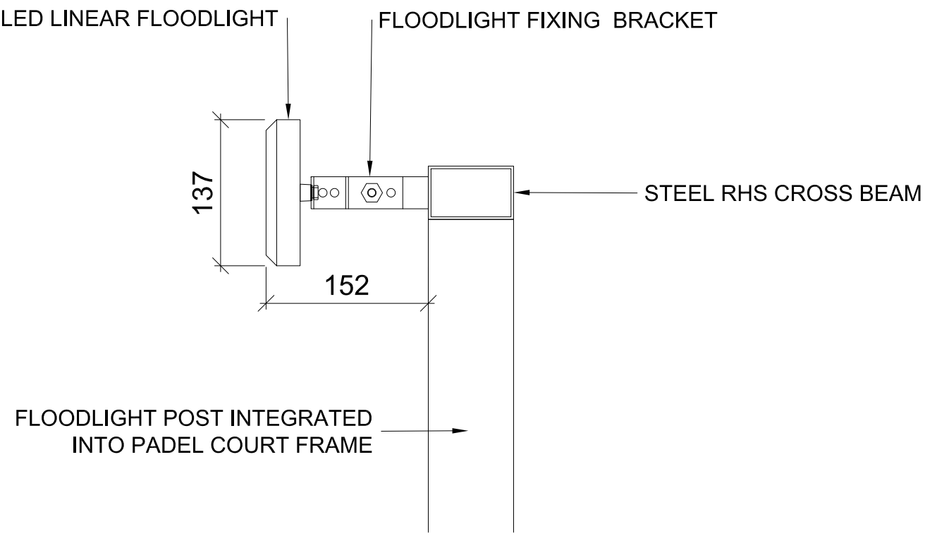
SIDE VIEW
