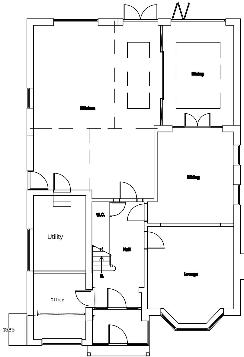
PROPOSED GND. FLOOR PLAN
