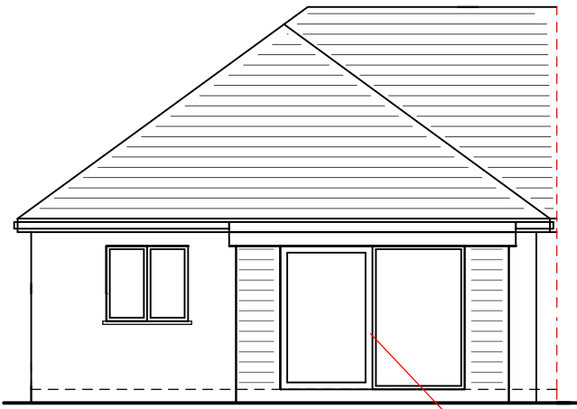
rear (east) elevation
