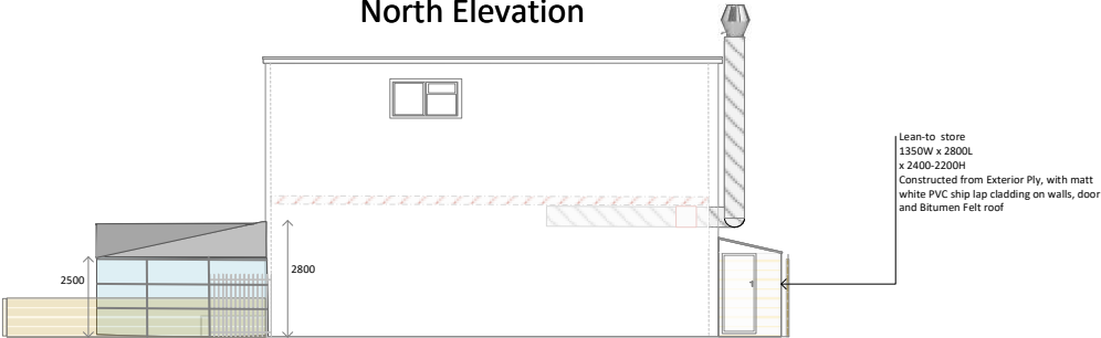
North Elevation
