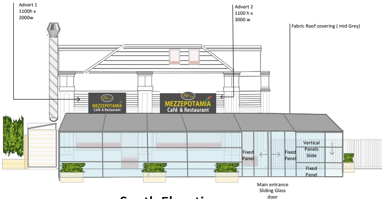
South Elevation
