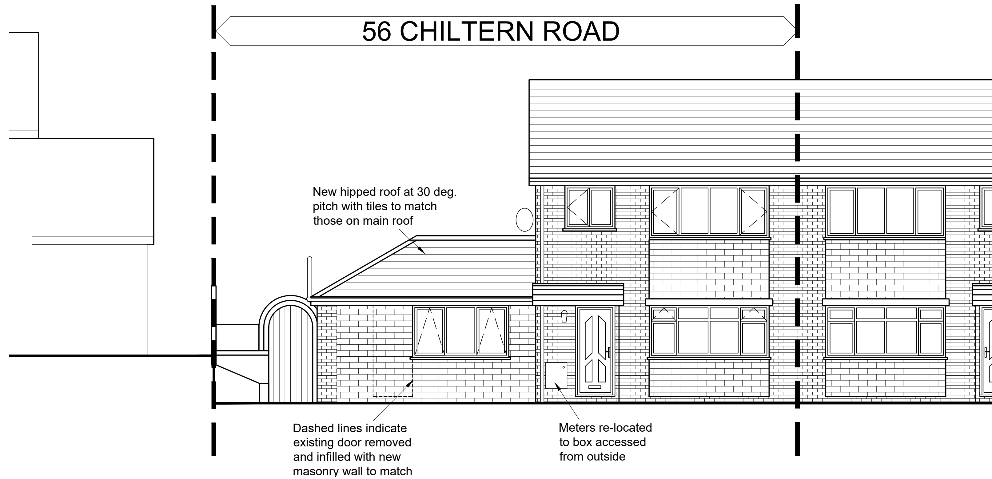
FRONT ELEVATION
