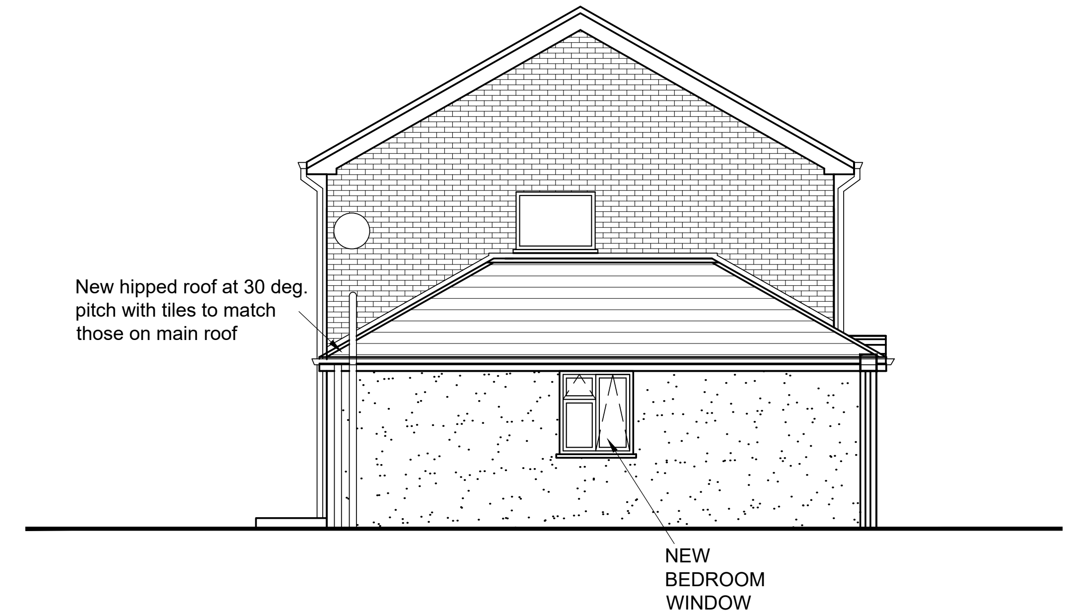
SIDE ELEVATION
