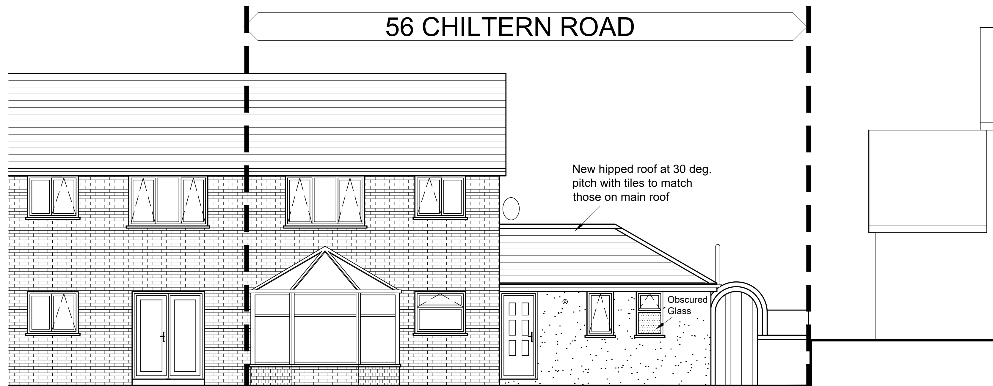
REAR ELEVATION
