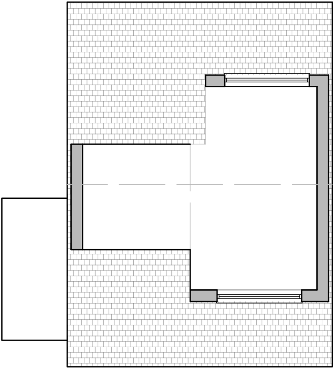
EXISTING LOFT PLAN
