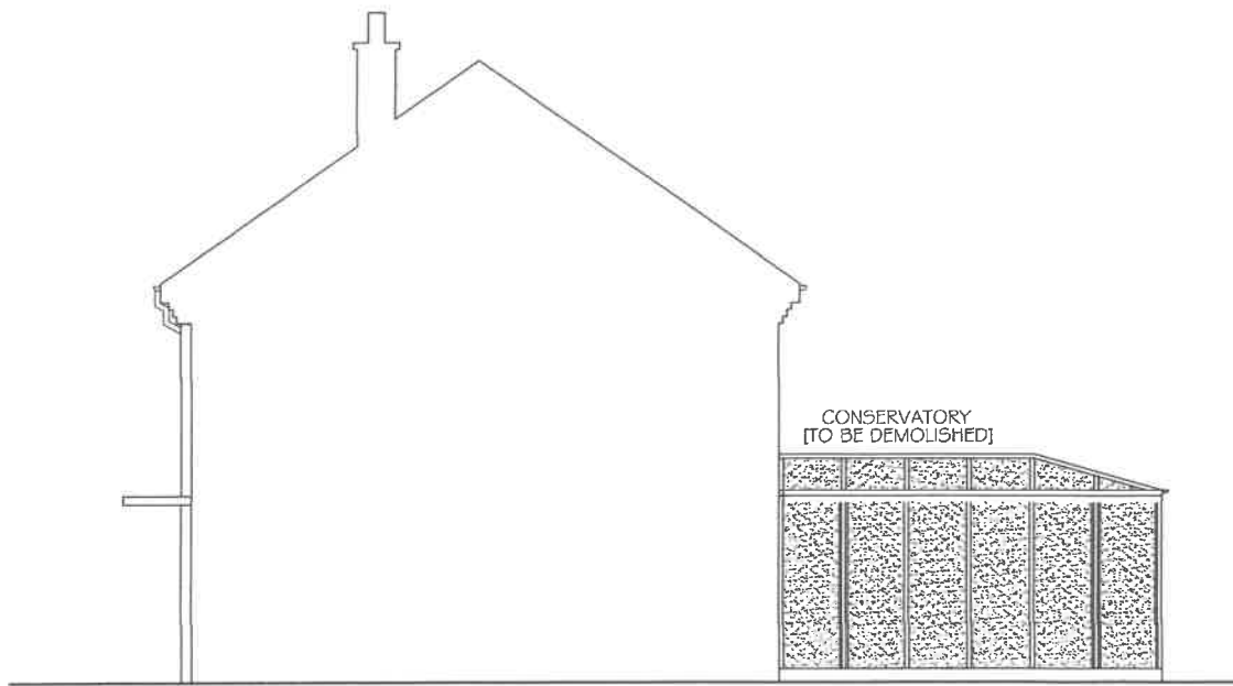
EXISTING NORTH EAST ELEVATION/SECTION [VIEWED FROM NO. 110] 1:100
