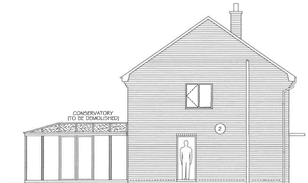
EXISTING SOUTH WEST ELEVATION 1:100
