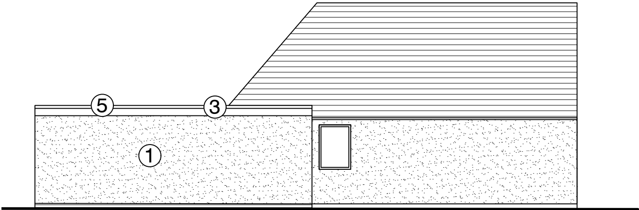
PROPOSED GABLE 2 ELEVATION
