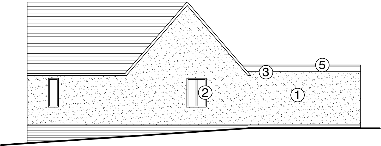
PROPOSED GABLE 1 ELEVATION
