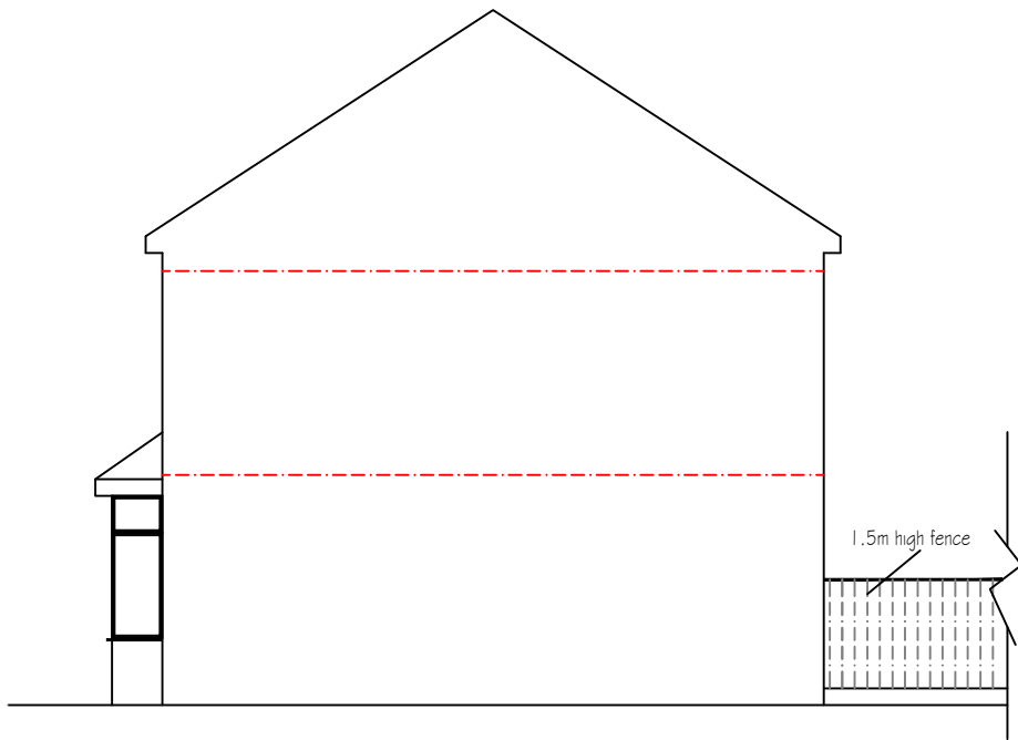
Elevation From No 10
