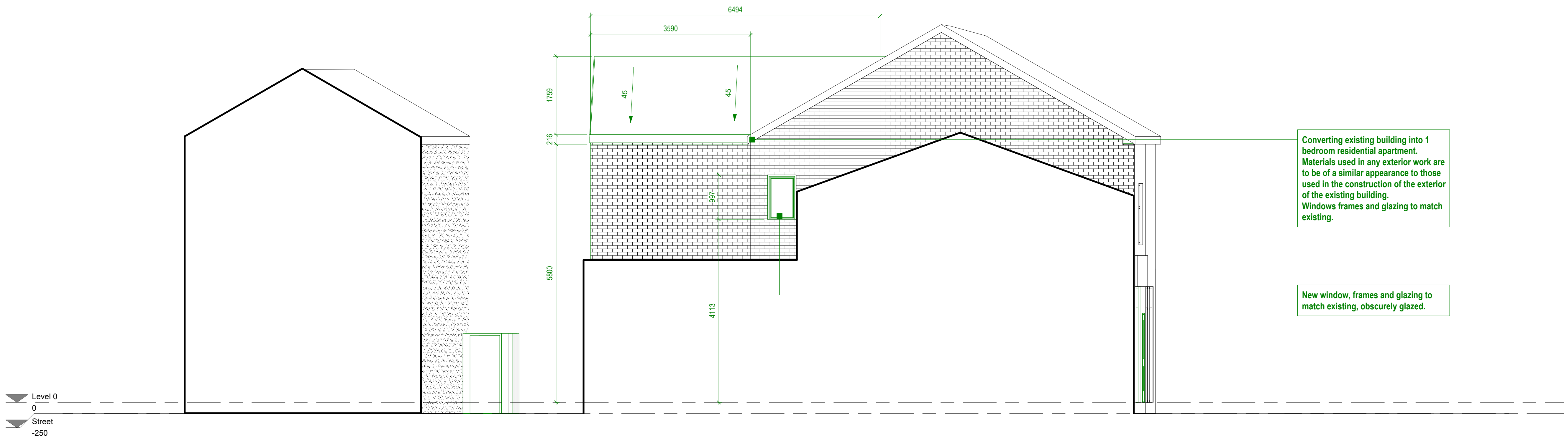
2 Proposed Side 1 Elevation 1 : 50
