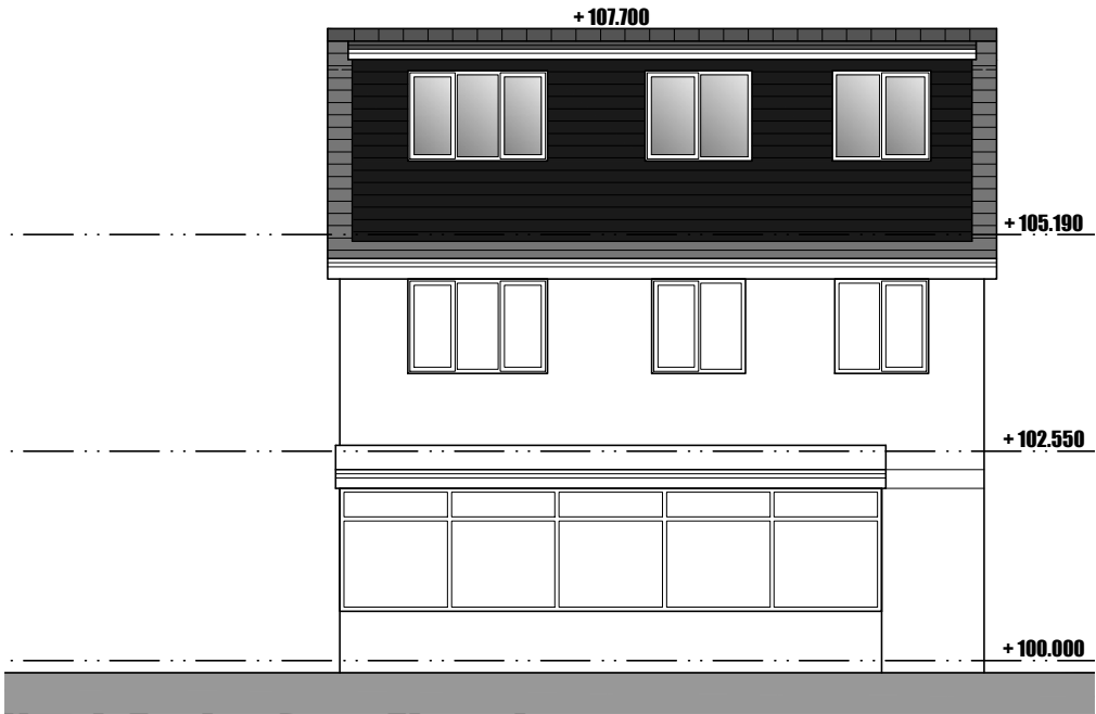
North Facing Rear Elevation
