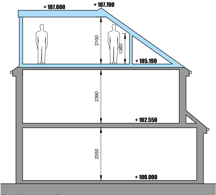
GA Cross Section
