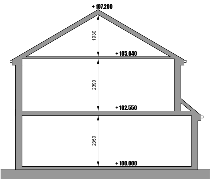
GA Cross Section
