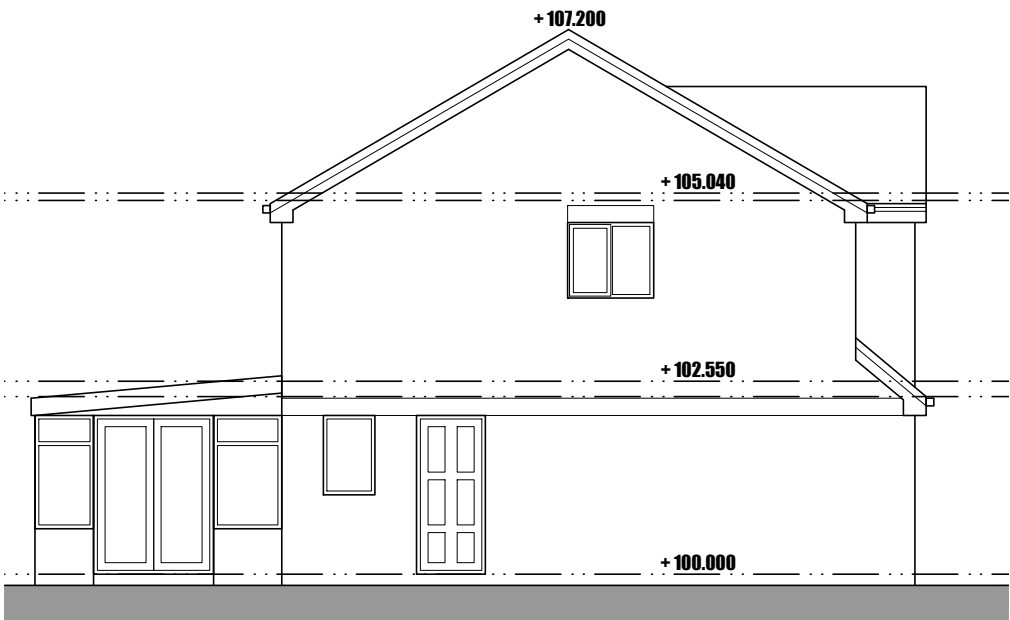
West Facing Side Elevation
