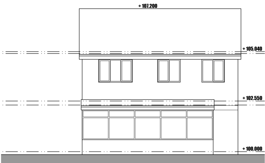
North Facing Rear Elevation
