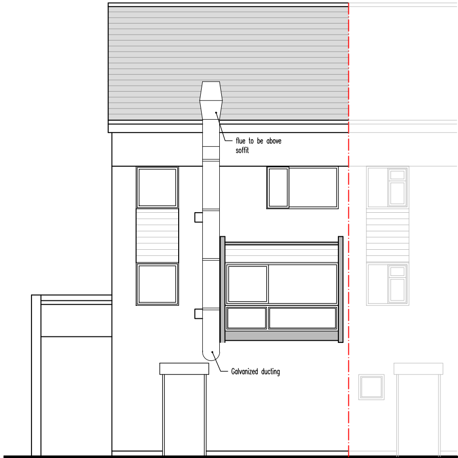
REAR ELEVATION
