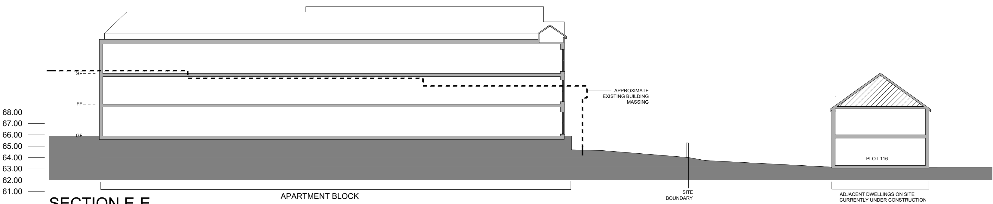
SECTION E-E
