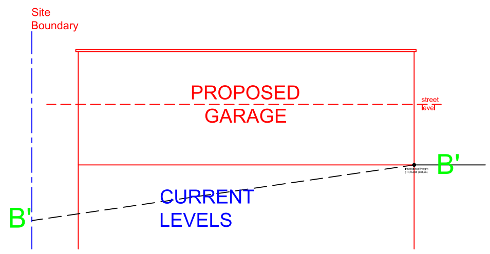
SECTION B-B' (see Dwg. No. 015A) As Existing & As Proposed) 1:100
