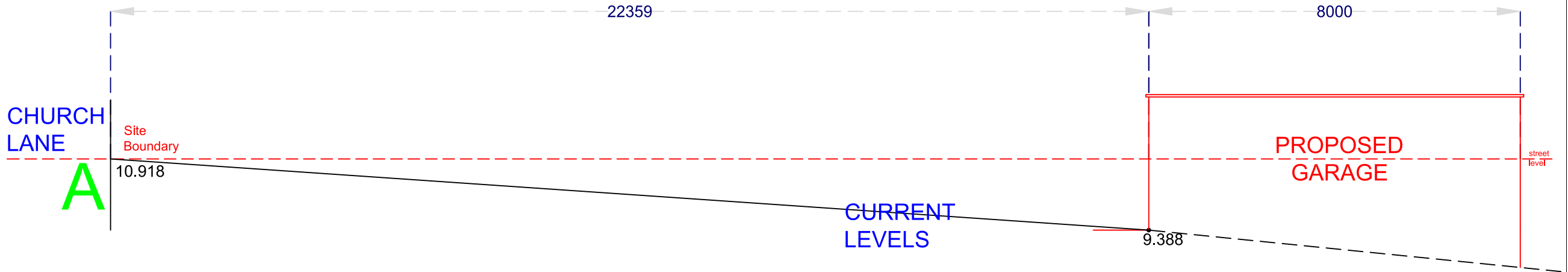
SECTION A-A' (see Dwg. No. 015A) As Existing & As Proposed) 1:100
