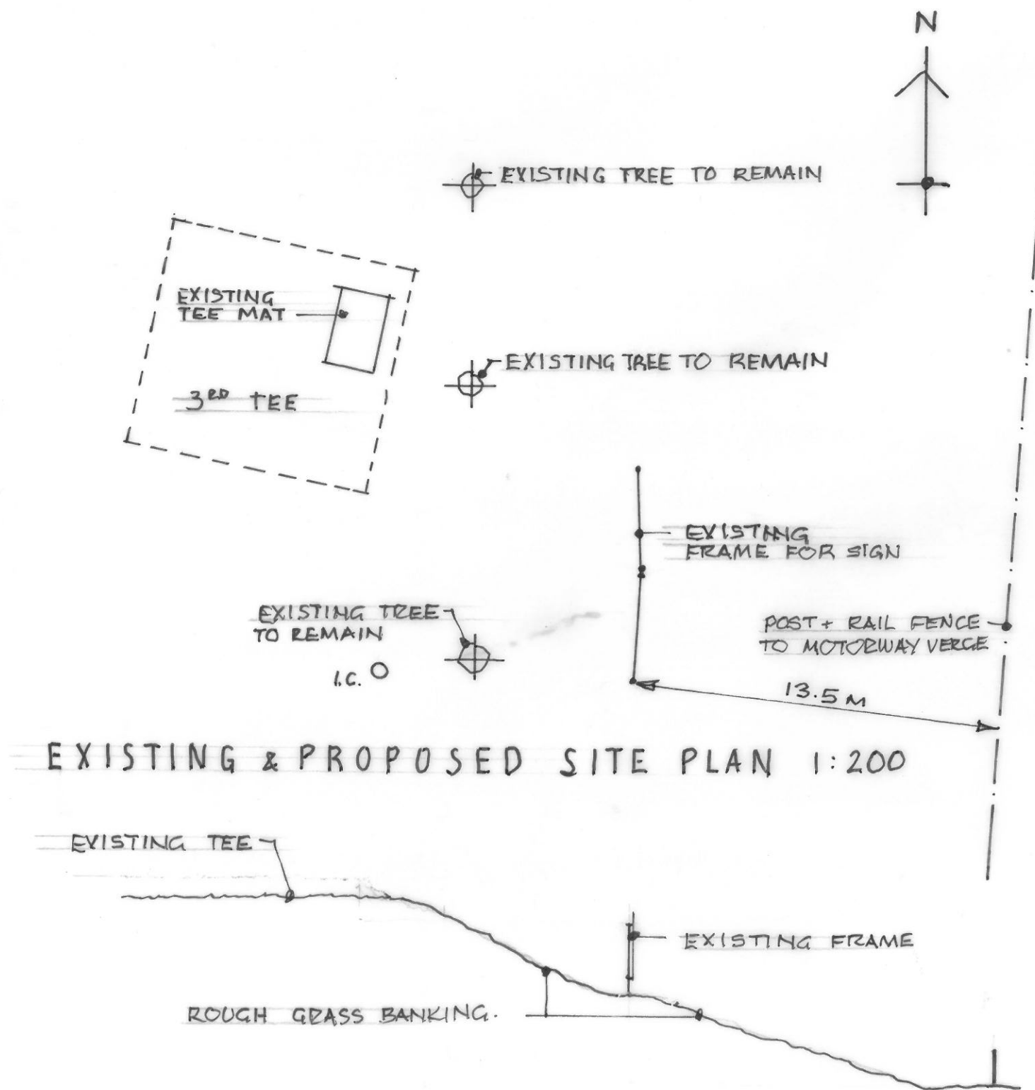
TYPICAL SECTION 1:200
