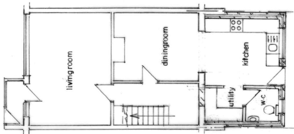
GROUND FLOOR PLAN (PROPOSED)
