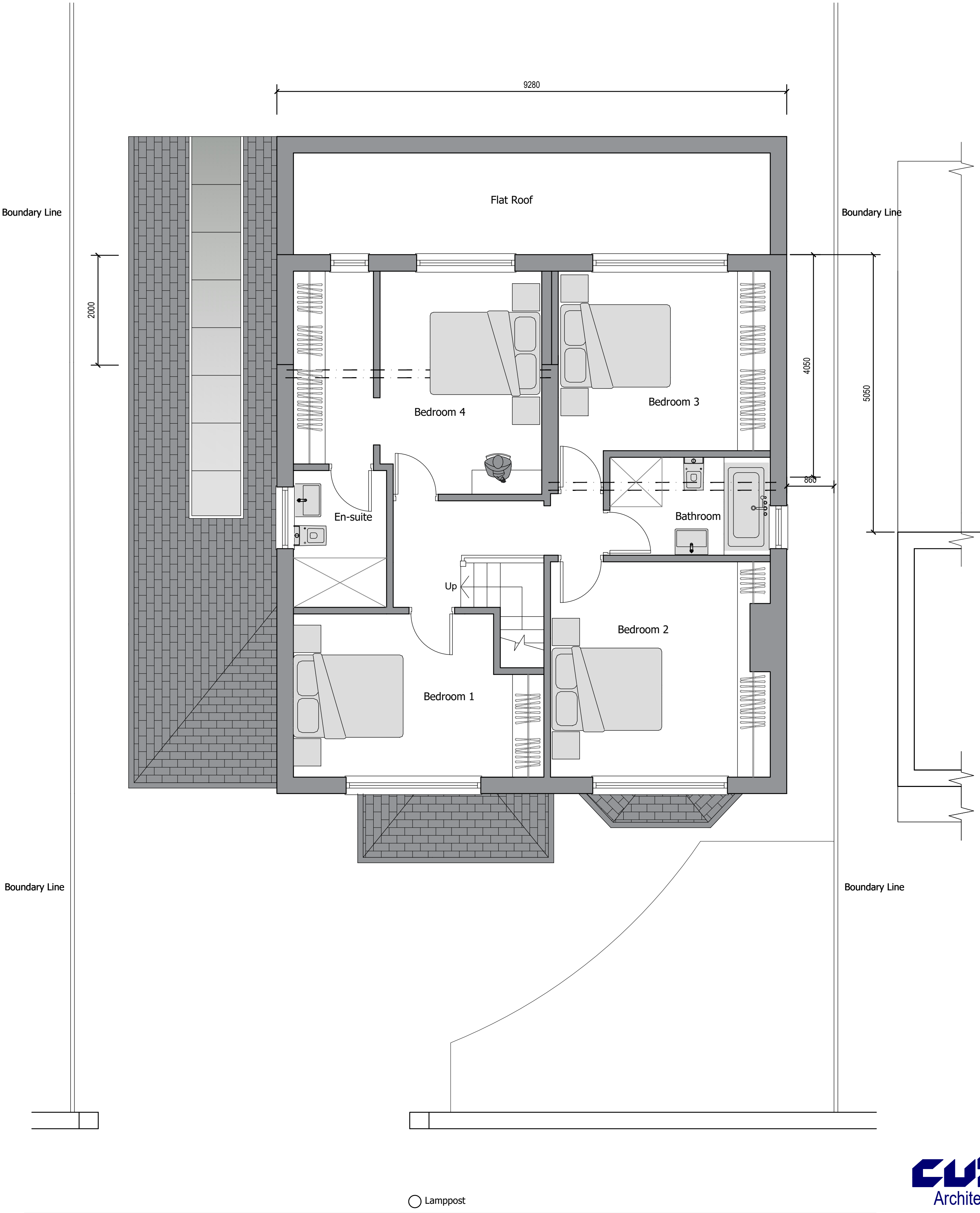
First Floor
