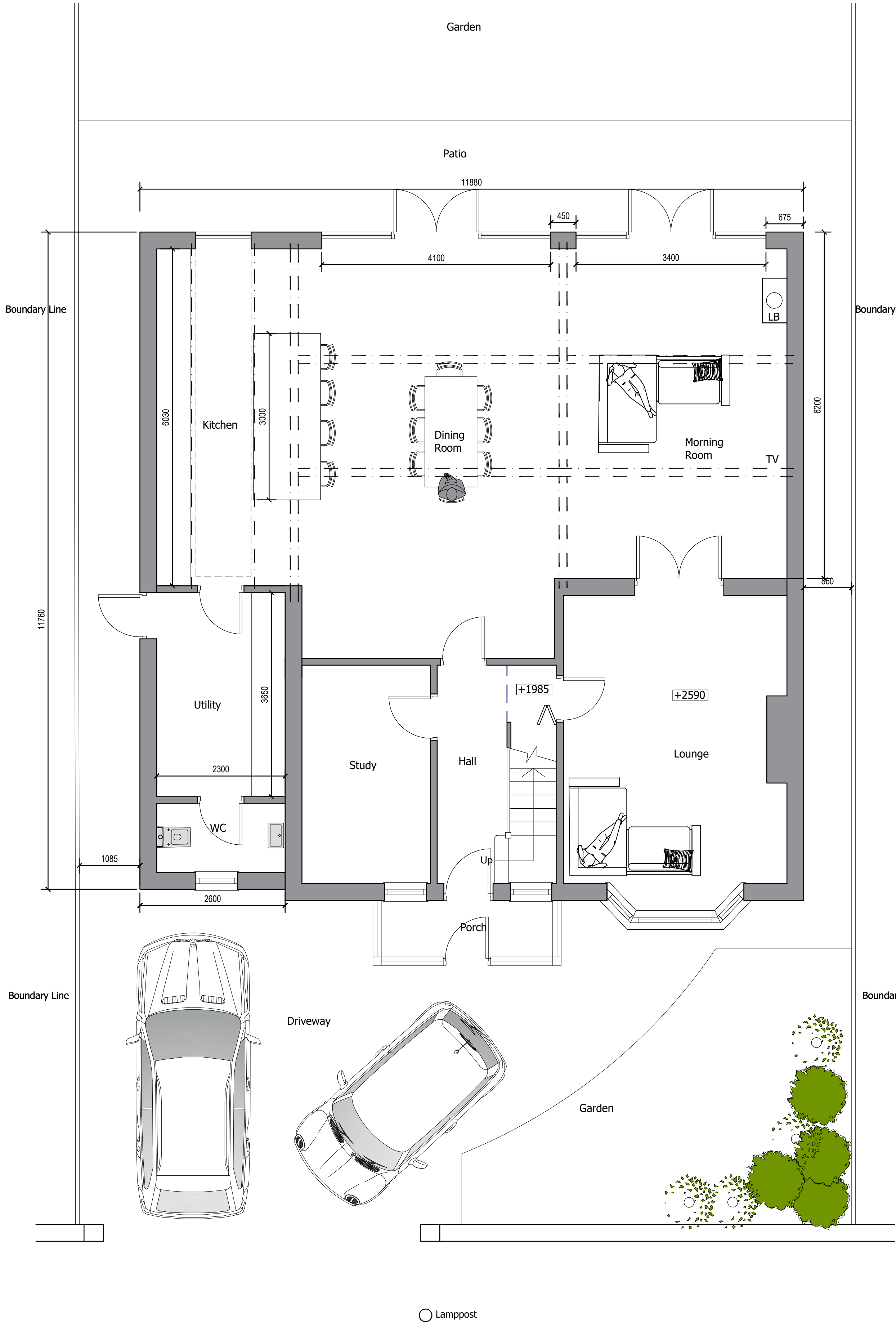
Ground Floor
