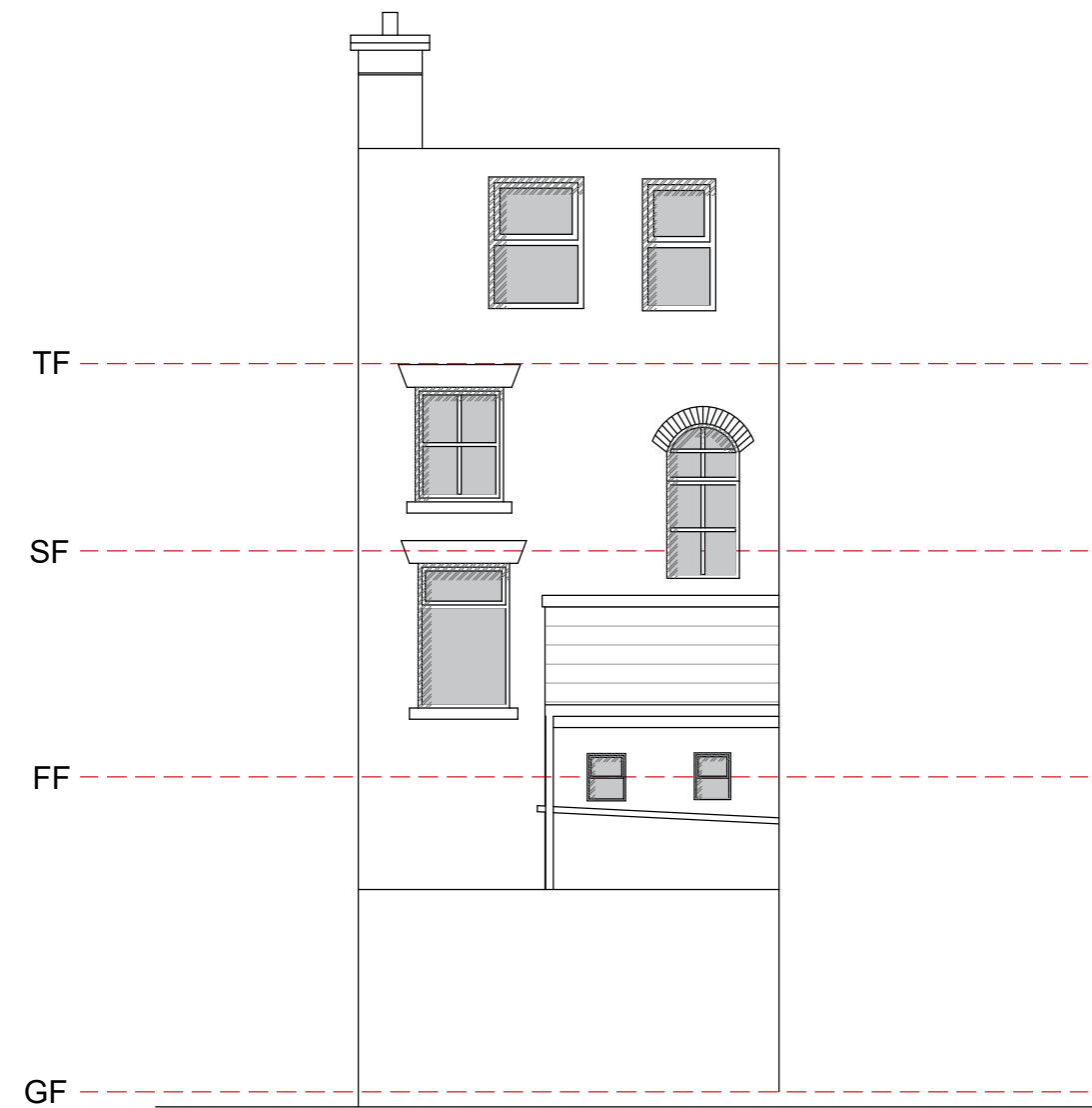
REAR ELEVATION
