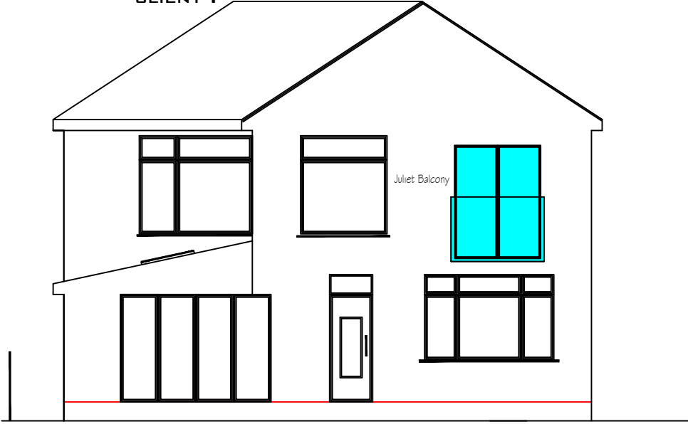
Rear Elevation
