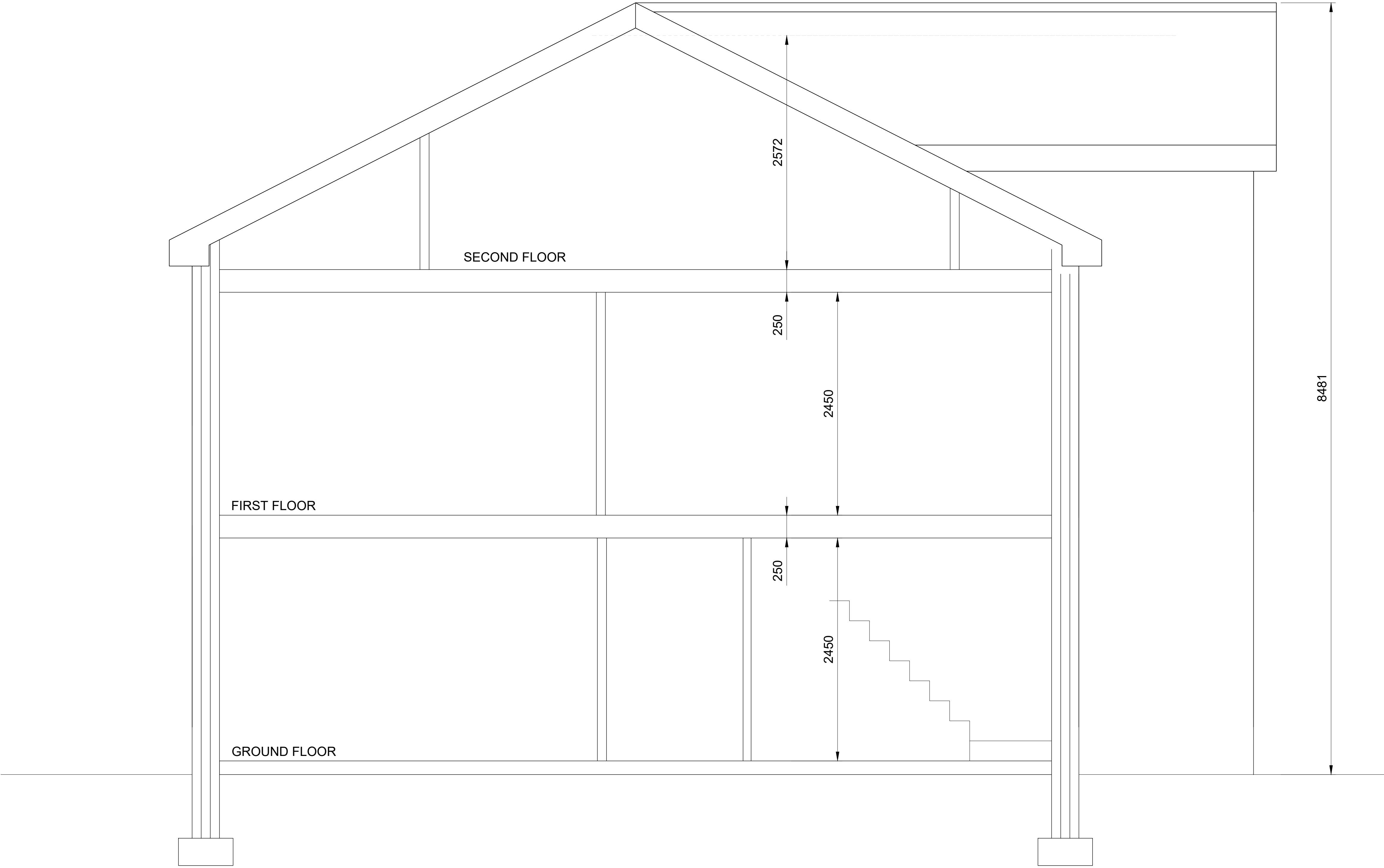
PROPOSED SECTION
