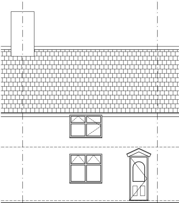
Existing South Elevation
