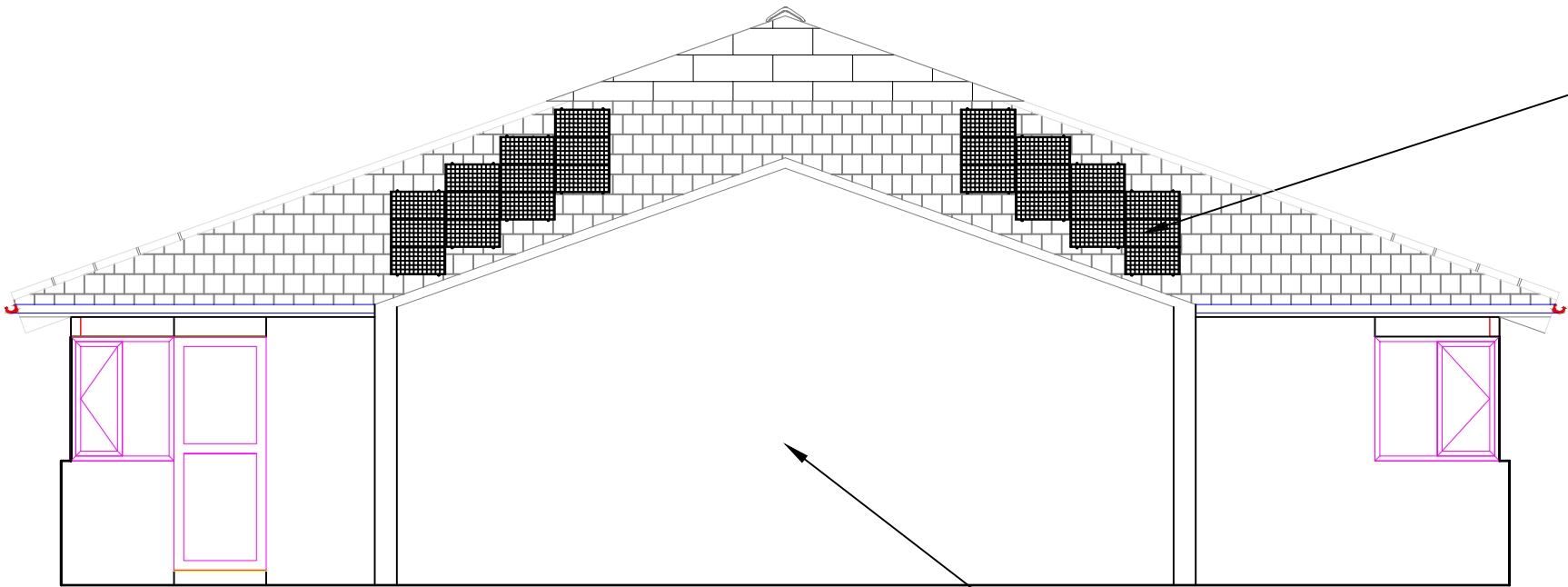
PROPOSED SOUTH-FACING ELEVATION DRAWING SHOWING THE SOLAR PV SUBJECT TO FINAL DESIGN LAYOUT.
