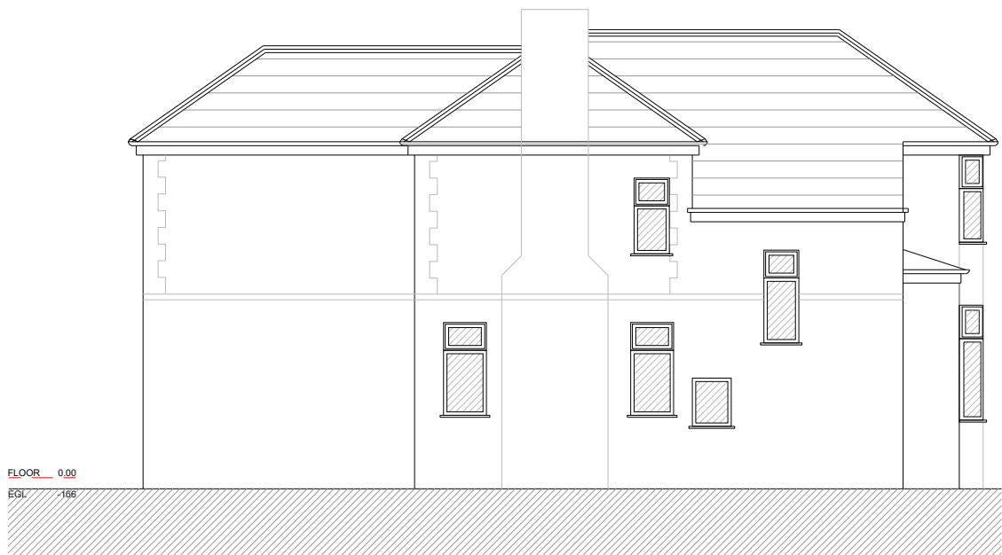
SIDE ELEVATION
