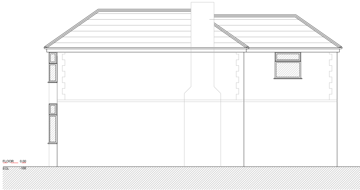
SIDE ELEVATION
