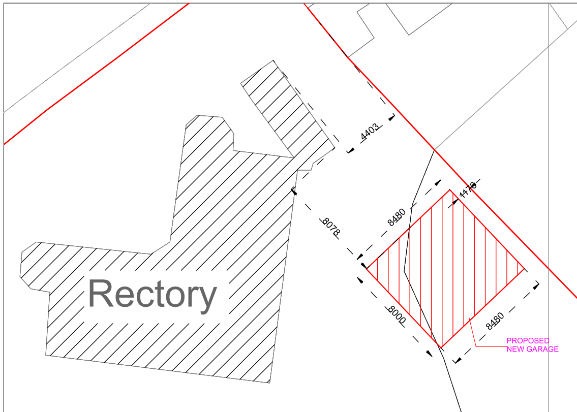
DETAILED SITE BLOCK PLAN 1:200
