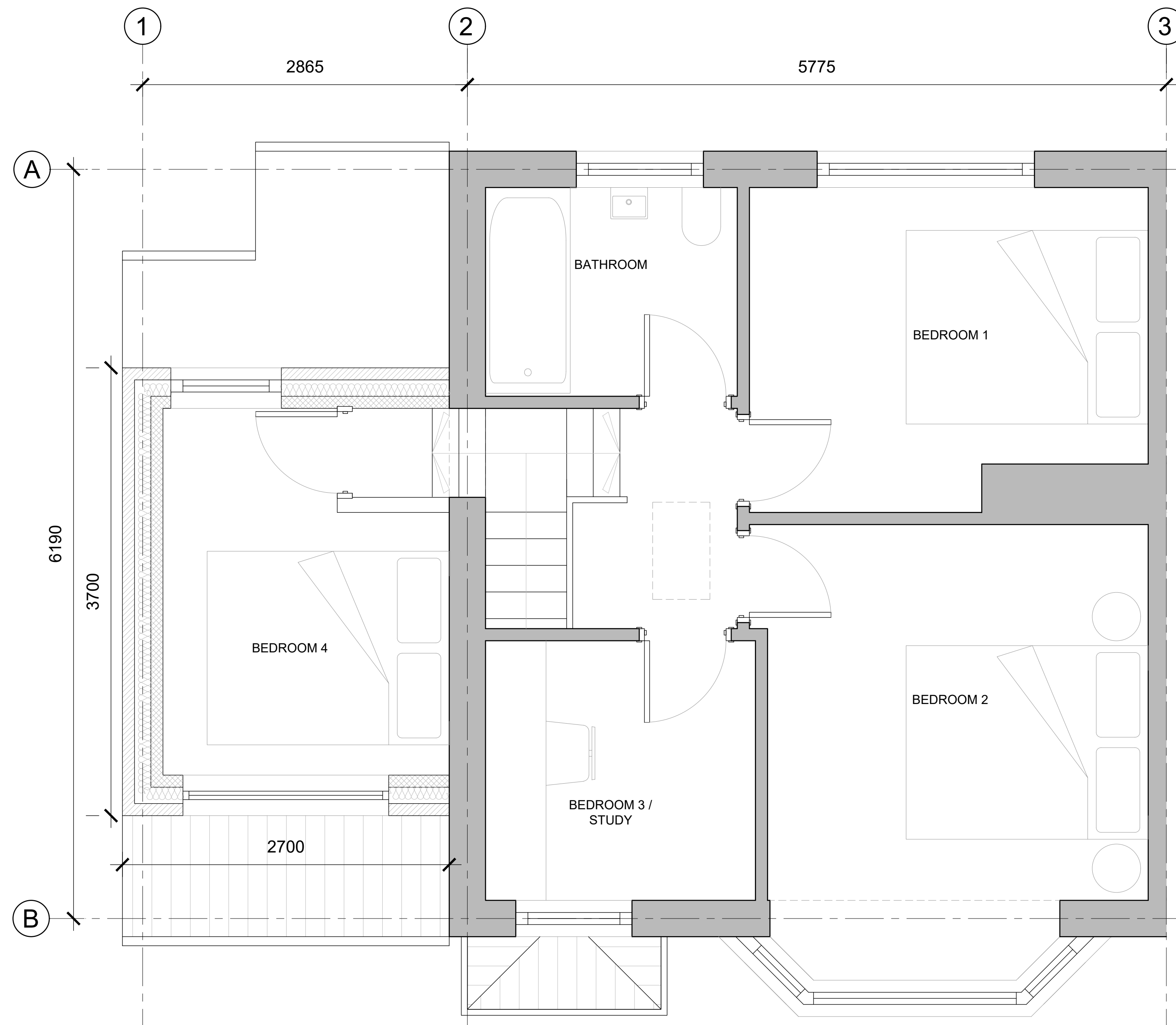
PROPOSED FIRST FLOOR
