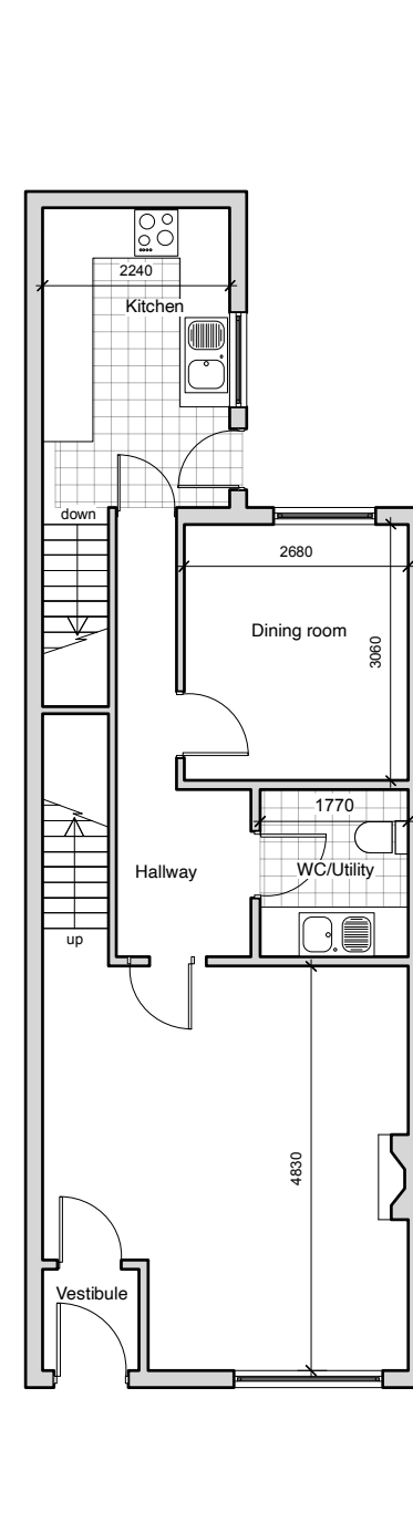
EXISTING GROUND FLOOR PLAN
