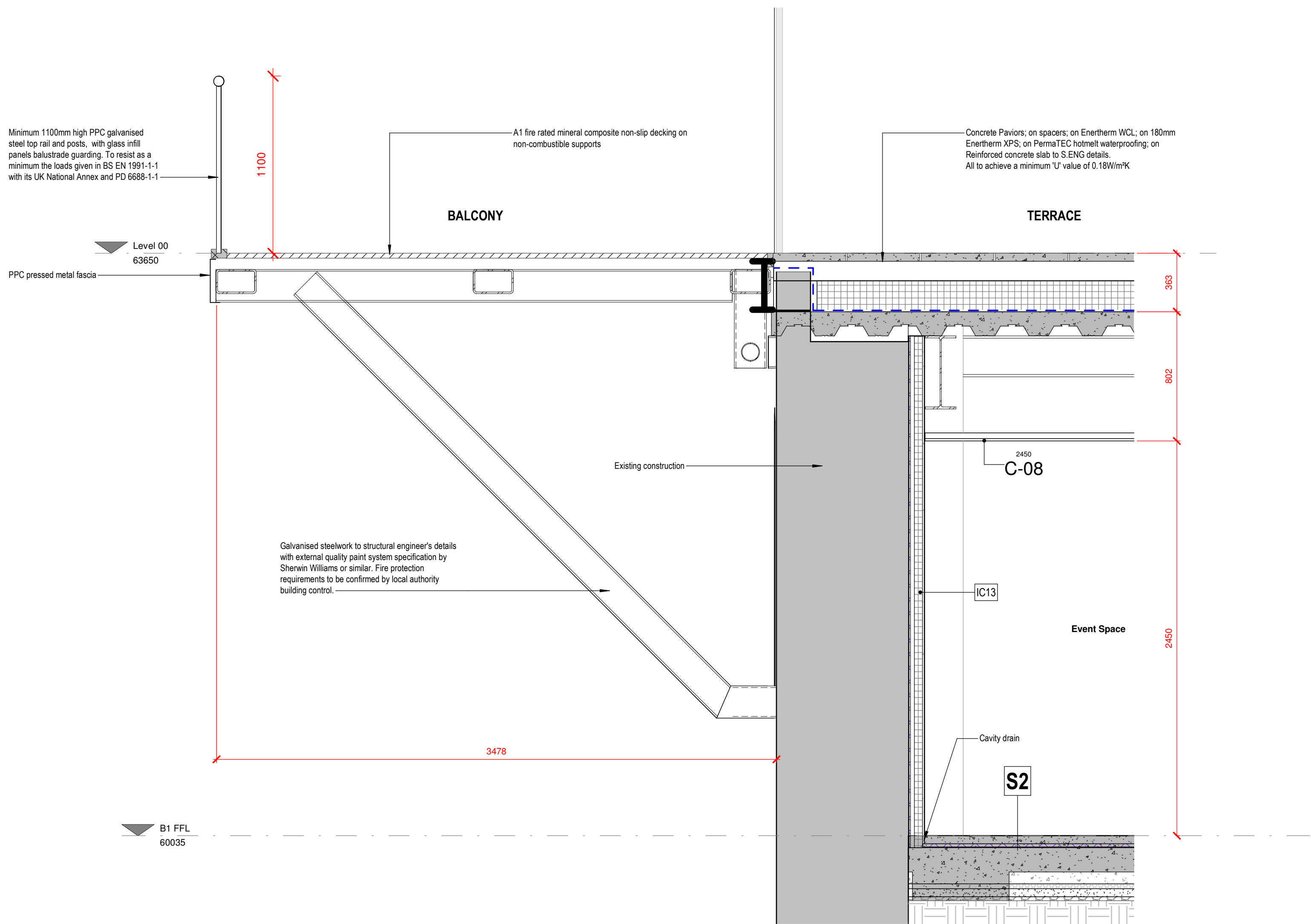
1 STRIP SECTION - Chamber Terrace 1 : 20
