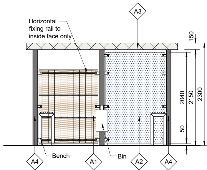
FRONT ELEVATION
