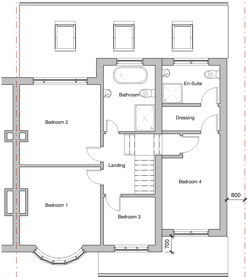
First Floor Proposed Plan 1 : 100
