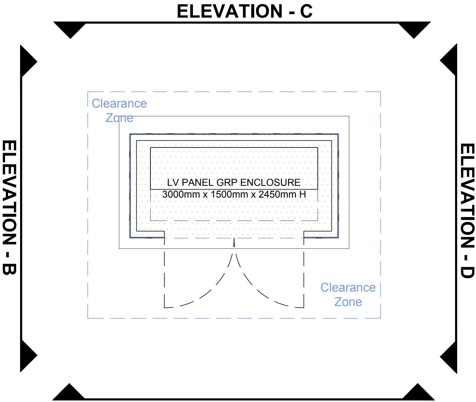
LV Enclosure Plan Scale 1:20
