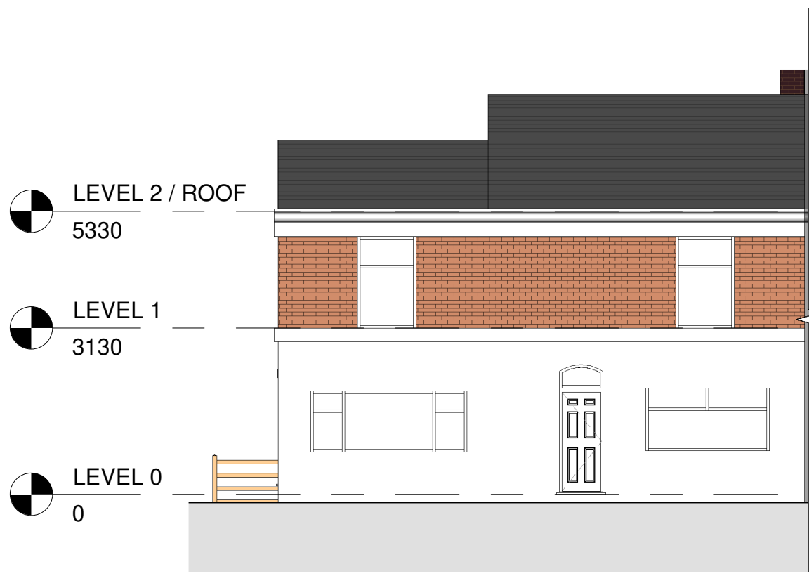
1 Front - Existing 1 : 100
