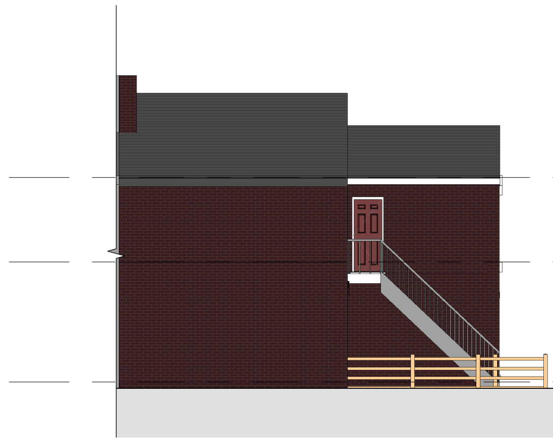
7 Rear - Proposed 1 : 100
