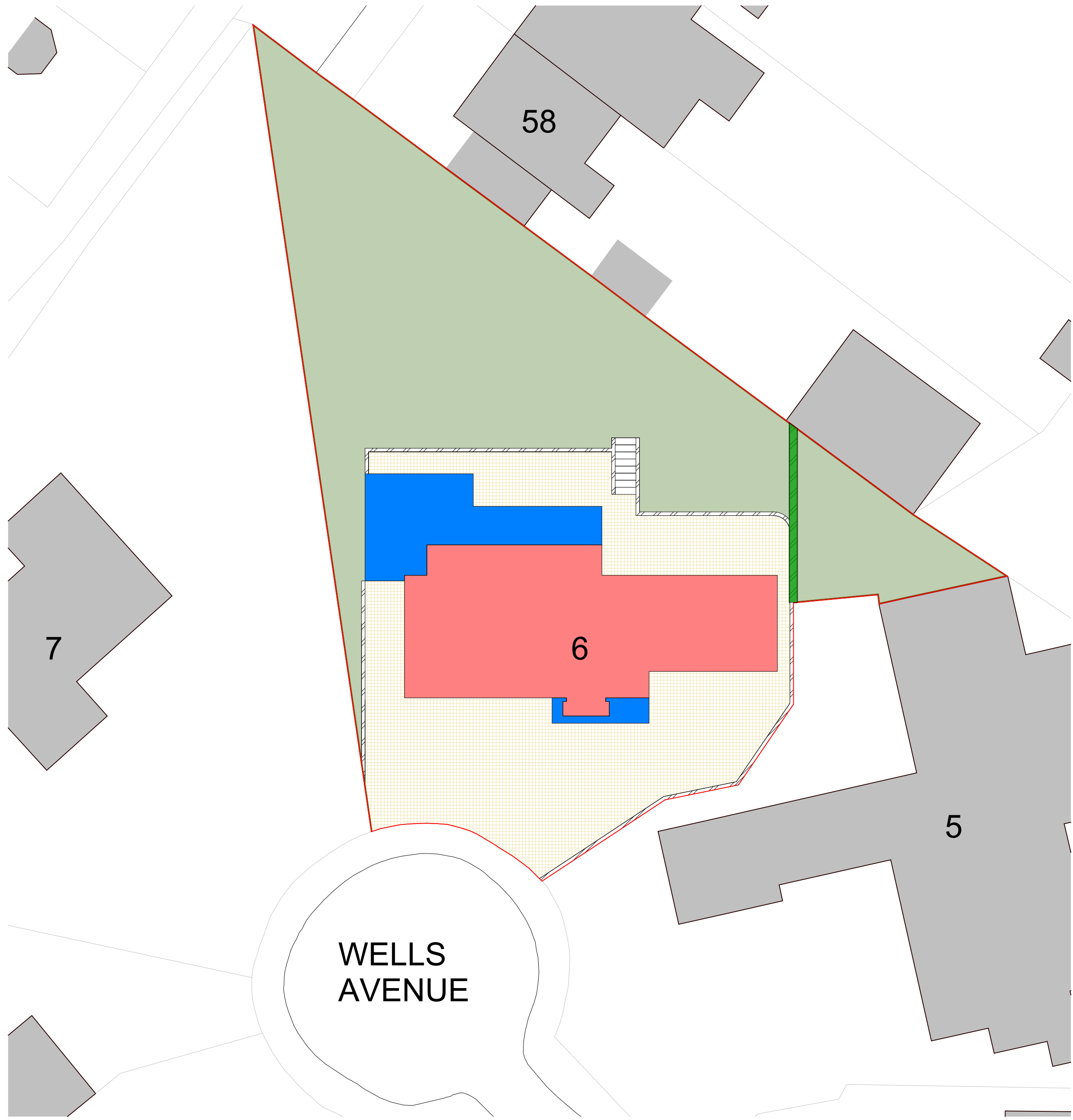
2 Site - Proposed 1 : 200
