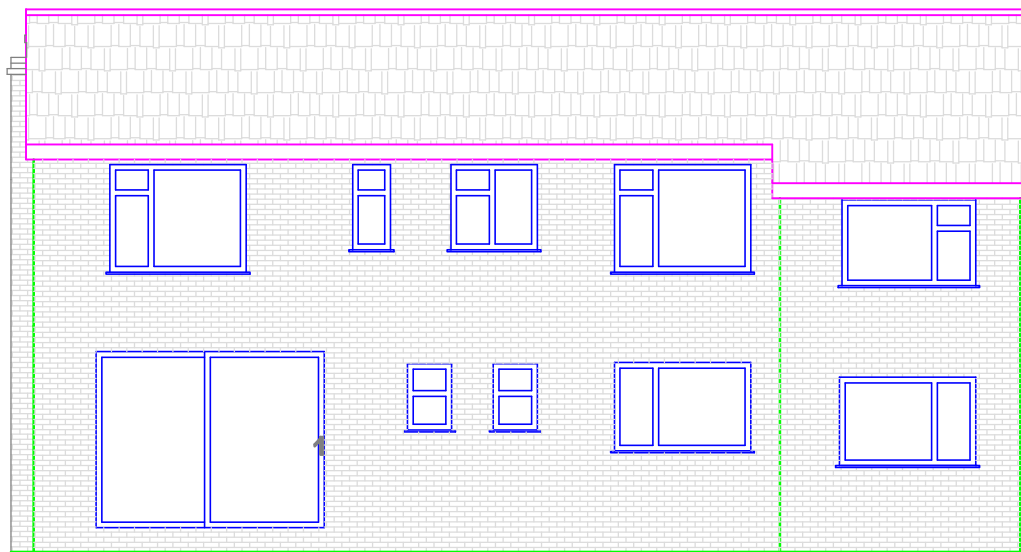
PROPOSED REAR ELEVATION (NO CHANGE)
