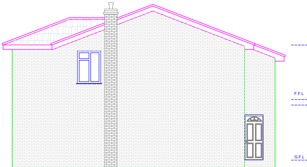
PROPOSED SIDE ELEVATION (NORTH WEST)
