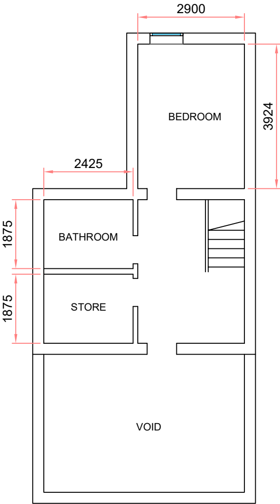
Proposed Basement Floor Plan
