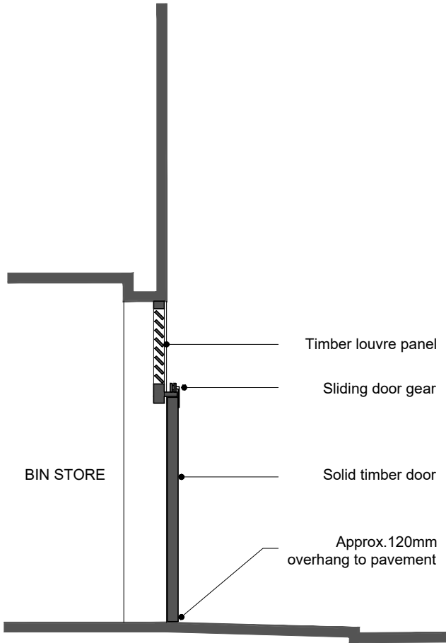
SECTIONAL DETAIL THROUGH SLIDING DOOR 1:50
