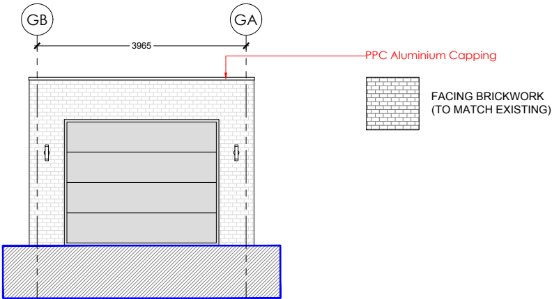
DETACHED GARAGE, FRONT ELEVATION 1:100
