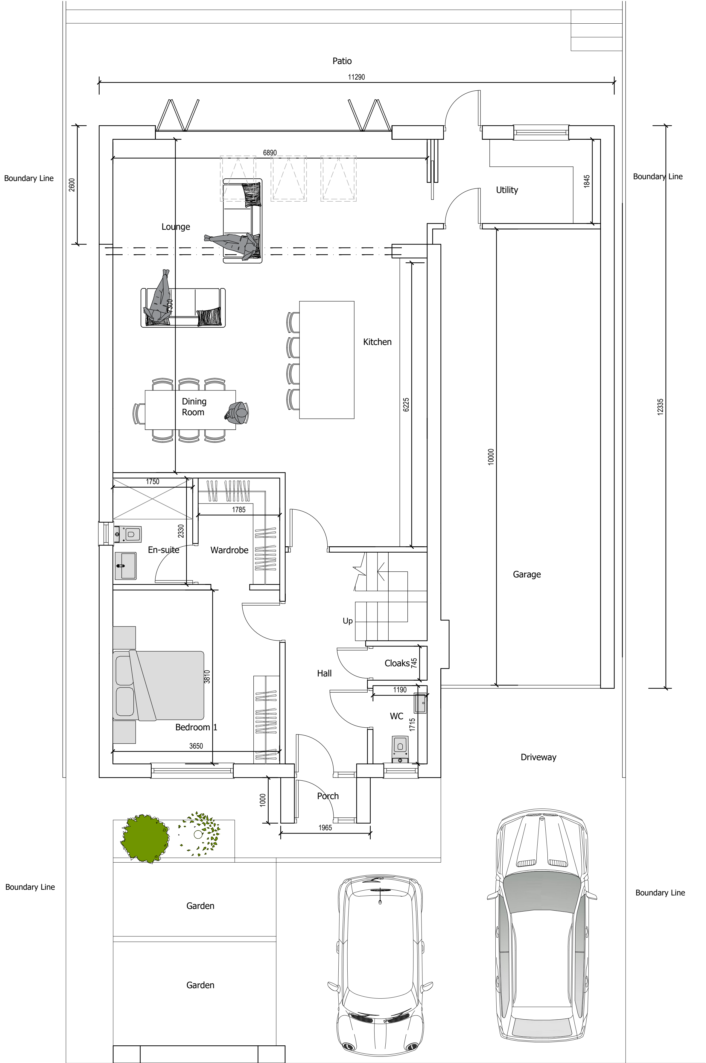
Ground Floor
