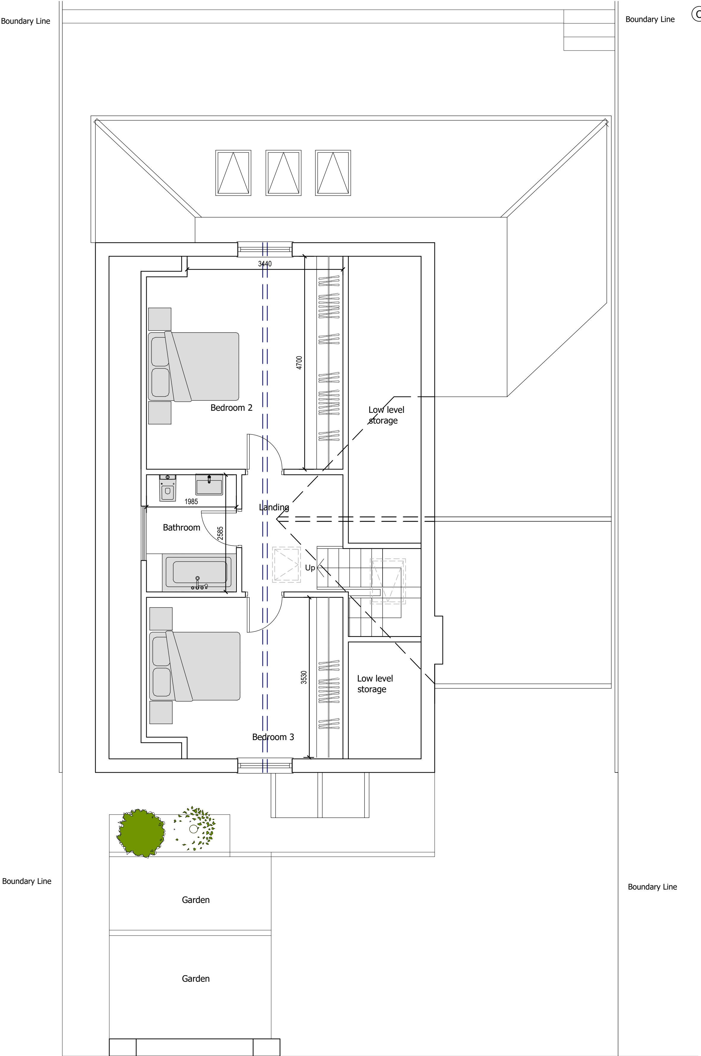
First Floor
