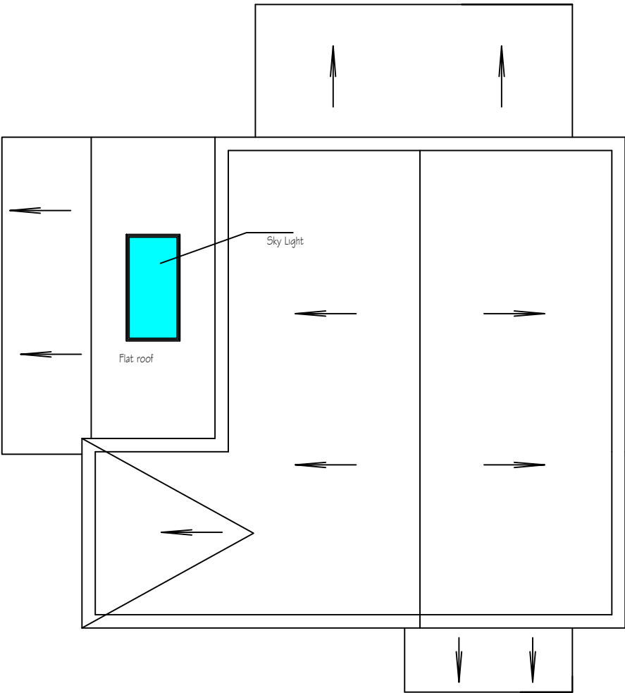
Roof Plan
