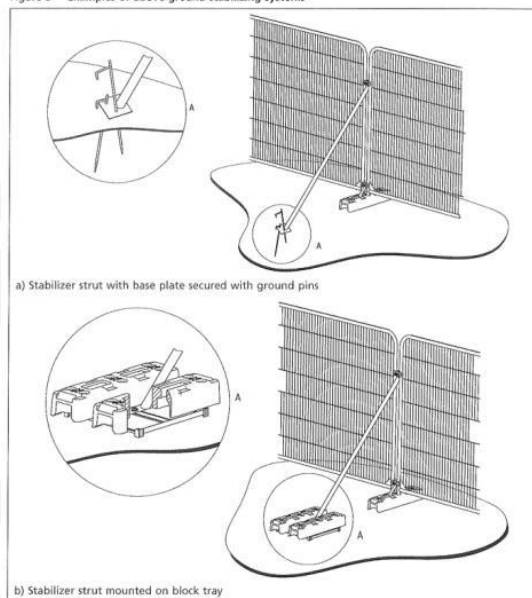
Figure 3 Examples of above-ground stabilizing systems
