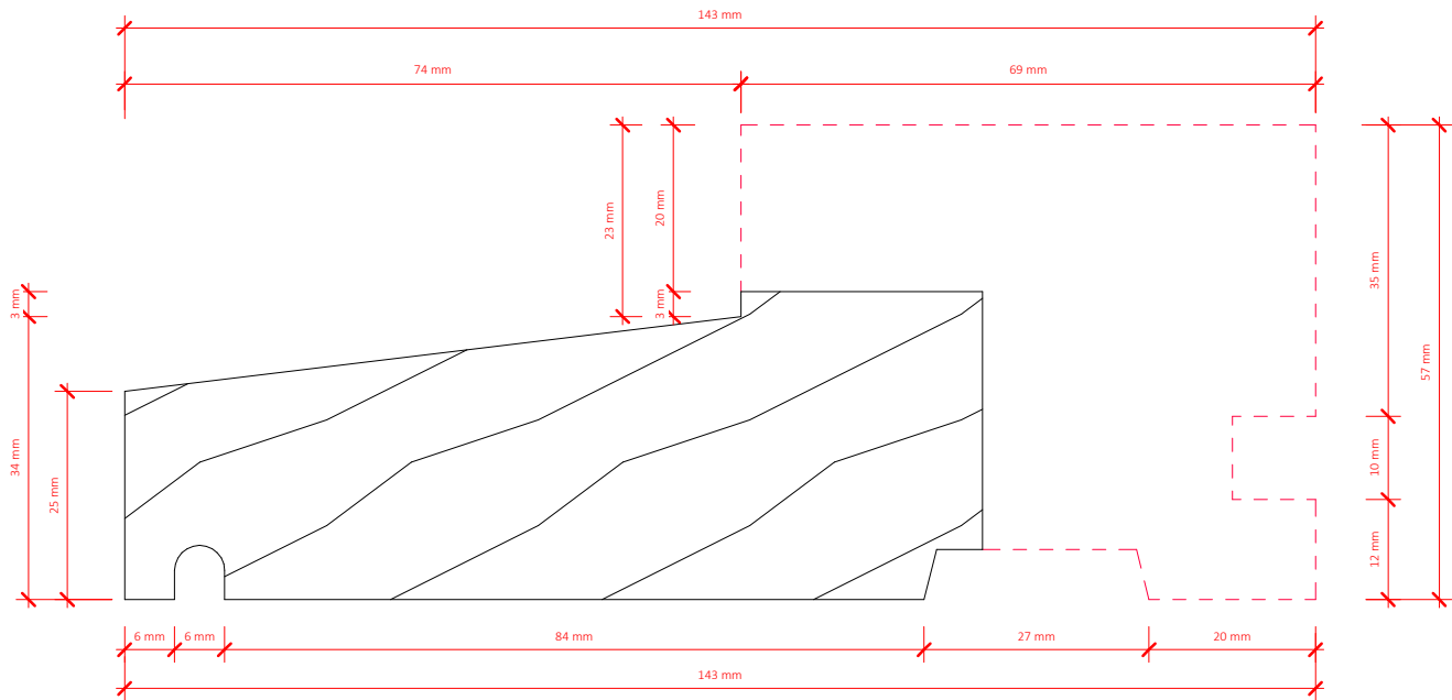
Mullion / Transom Profile (Pattern No. 348) Scale: 1:1
