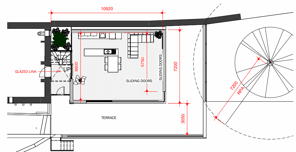
1 0 PROPOSED GROUND FLOOR 1 : 100
