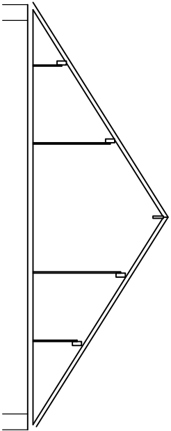
SECTION A-A THROUGH ROOF STRUCTURE 1:100.
