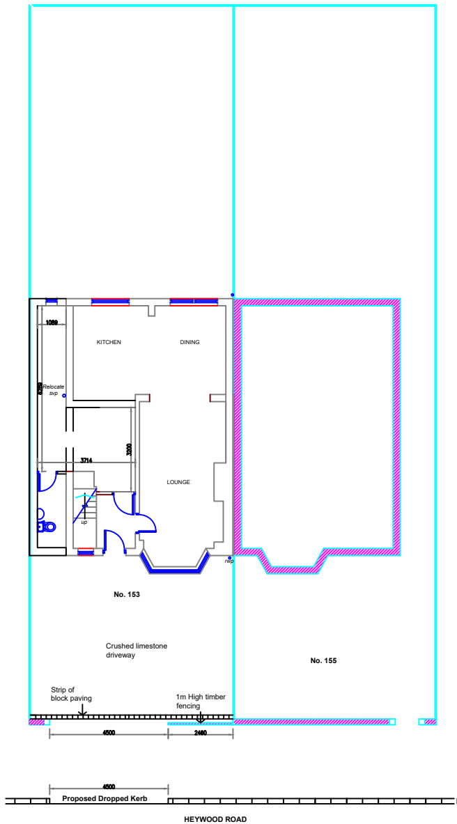
PROPOSED SITE PLAN 1:200
