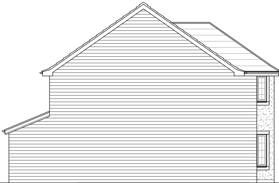
SIDE ELEVATION
