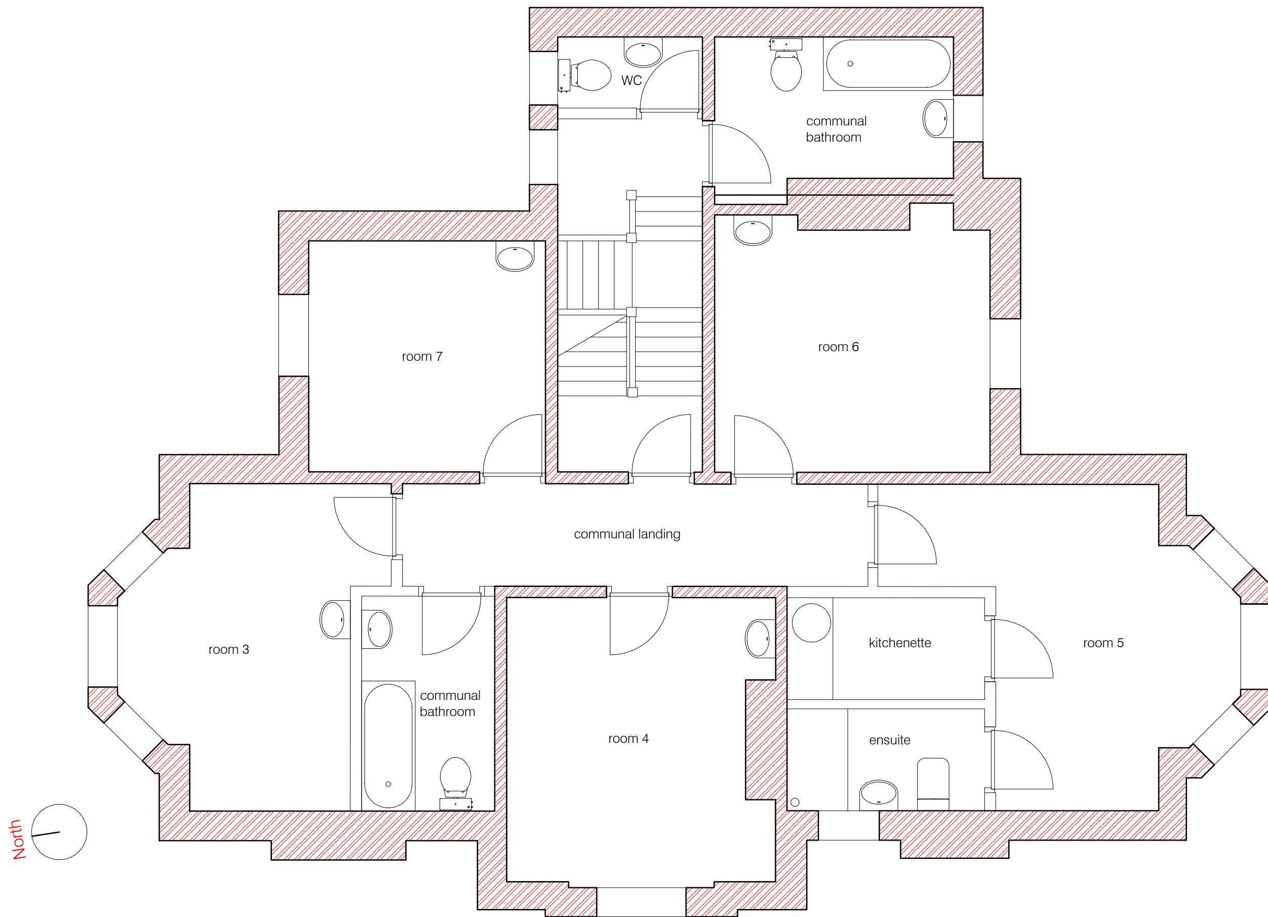
Existing First Floor Plan 1:50 @ A3 - Gross Internal Area = 101.7m 2
